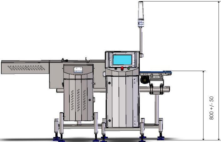
All Measurements in MM (Model Shown 1500UL)
